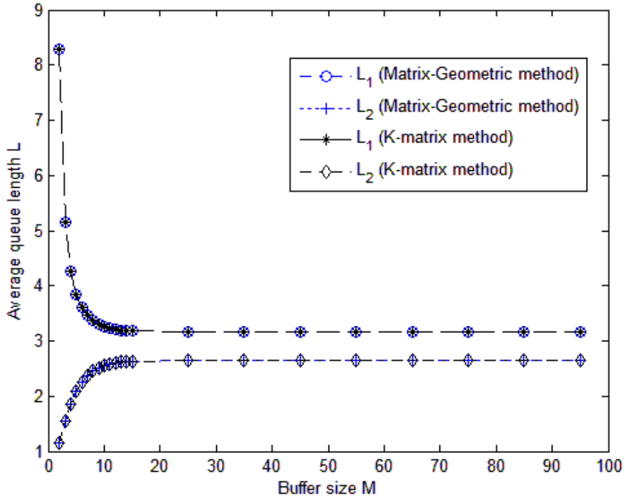
Figure 3. Average system size L_1 ( L_2 ) versus the buffer size M obtained by Matrix-Geometric method and K -matrix method with parameters \Lambda = 1 and \mu_f = \mu_c = 0.6 .
